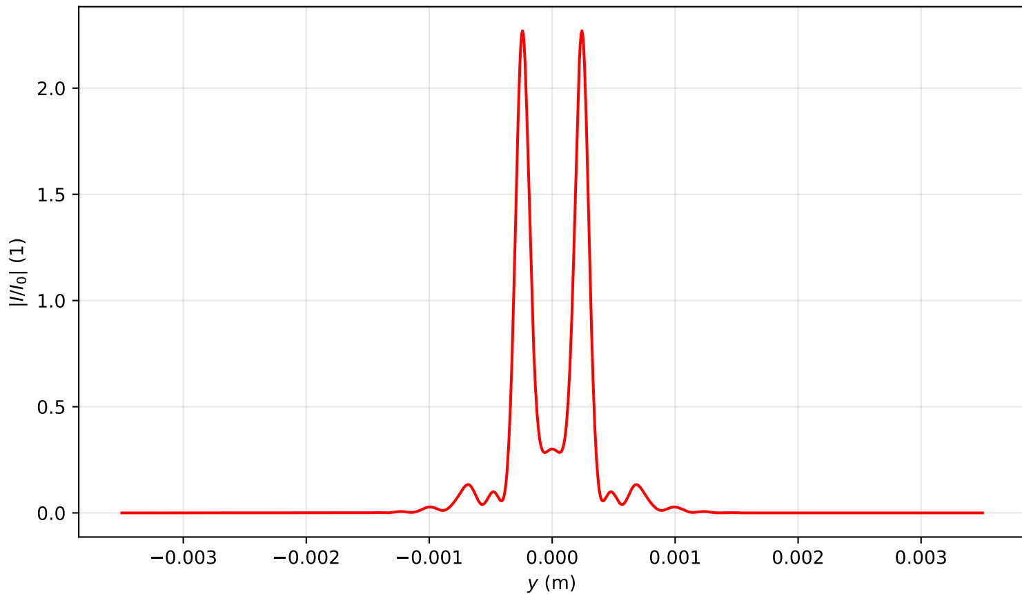
Intensity profile I(x=0, y, z=0.716)/I_0 , P_{in}=6.0P_{cr} , artificial time
